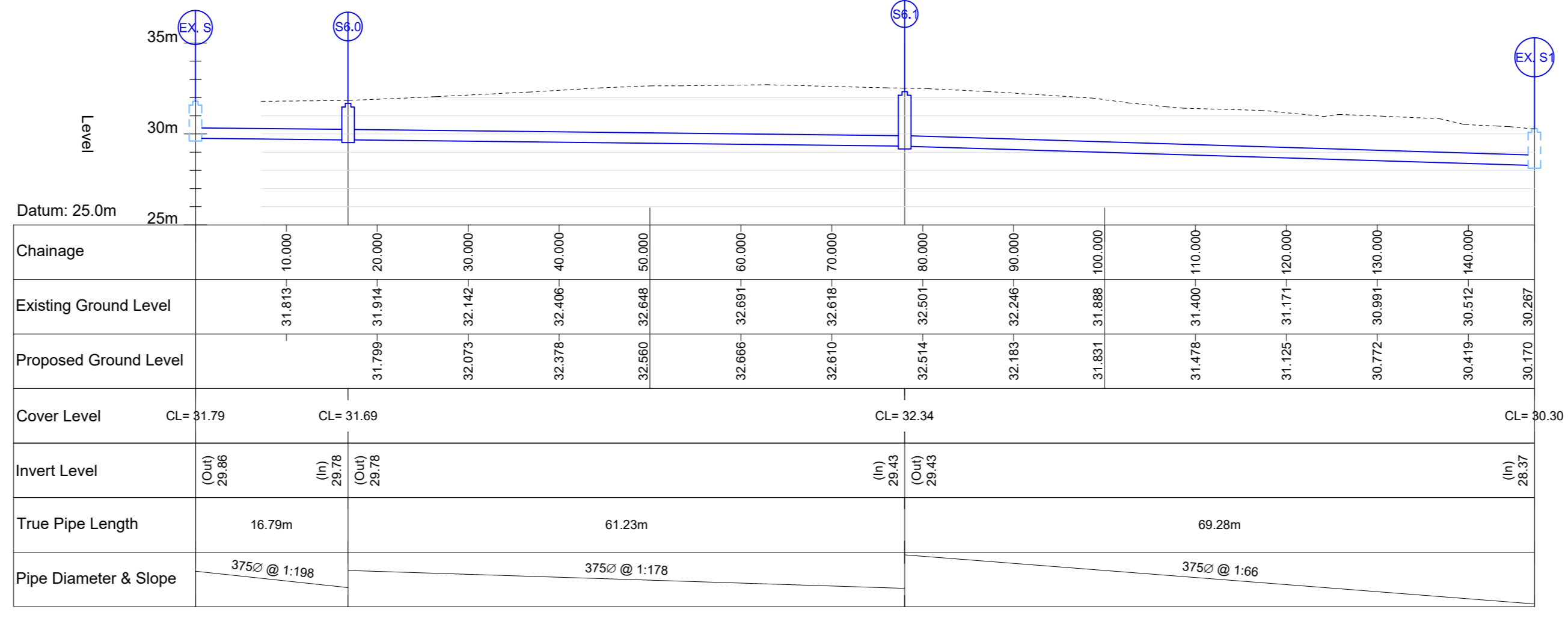
S6 SECTION SCALE @ A0: H=1:500, V=1:250 SCALE @ A2: H=1:1000, V=1:500
