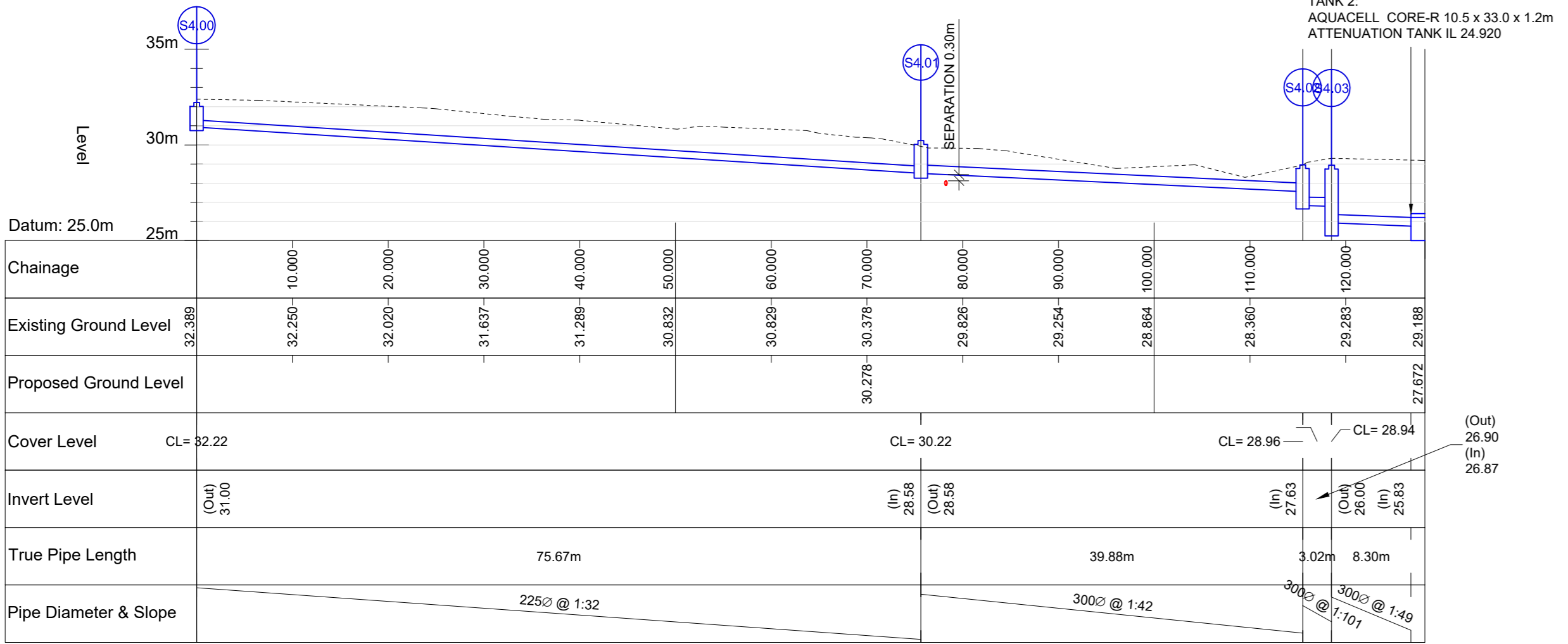
S4 SECTION SCALE @ A0: H=1:500, V=1:250 SCALE @ A2: H=1:1000, V=1:500
