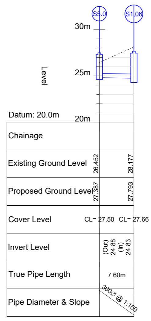
S5 SECTION SCALE @ A0: H=1:500, V=1:250 SCALE @ A2: H=1:1000, V=1:500
