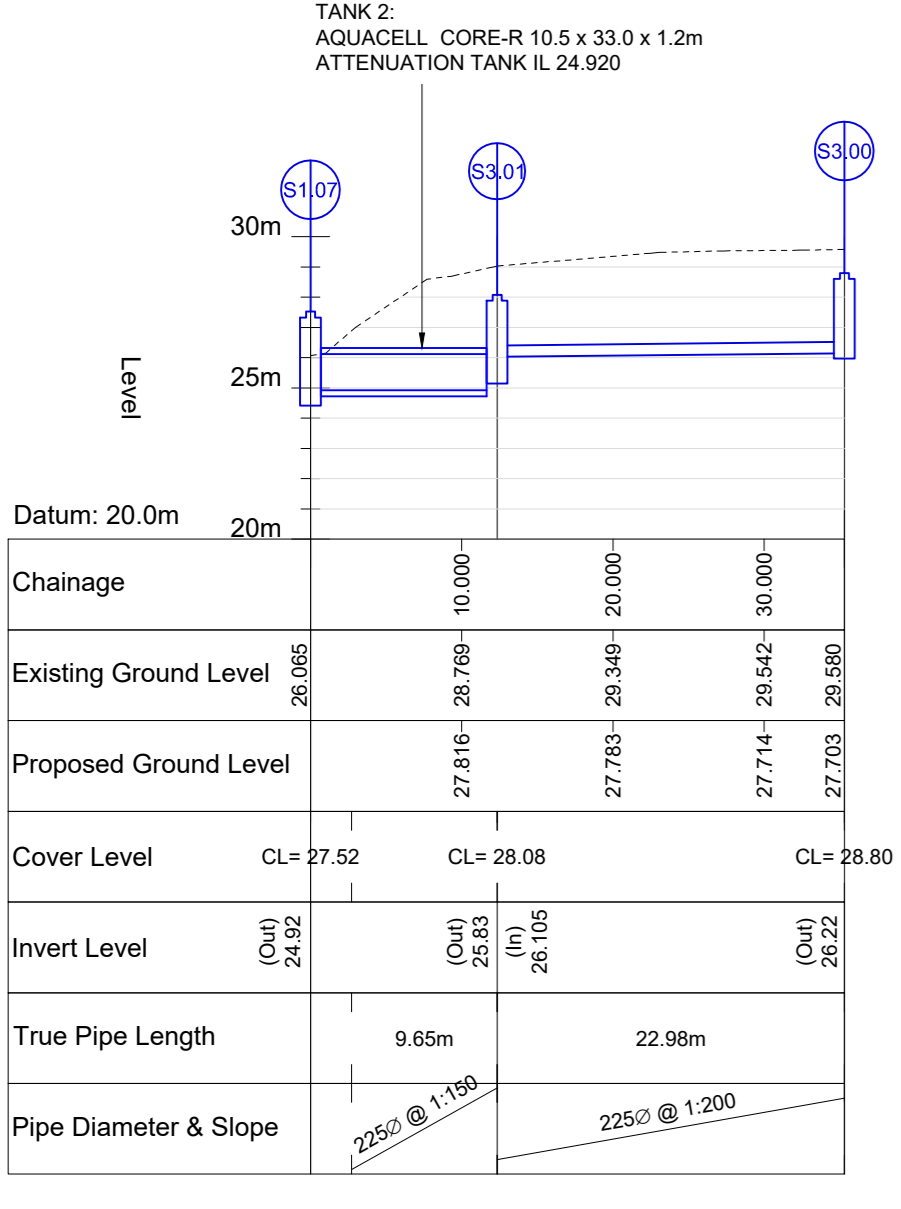
S3 SECTION SCALE @ A0: H=1:500, V=1:250 SCALE @ A2: H=1:1000, V=1:500
