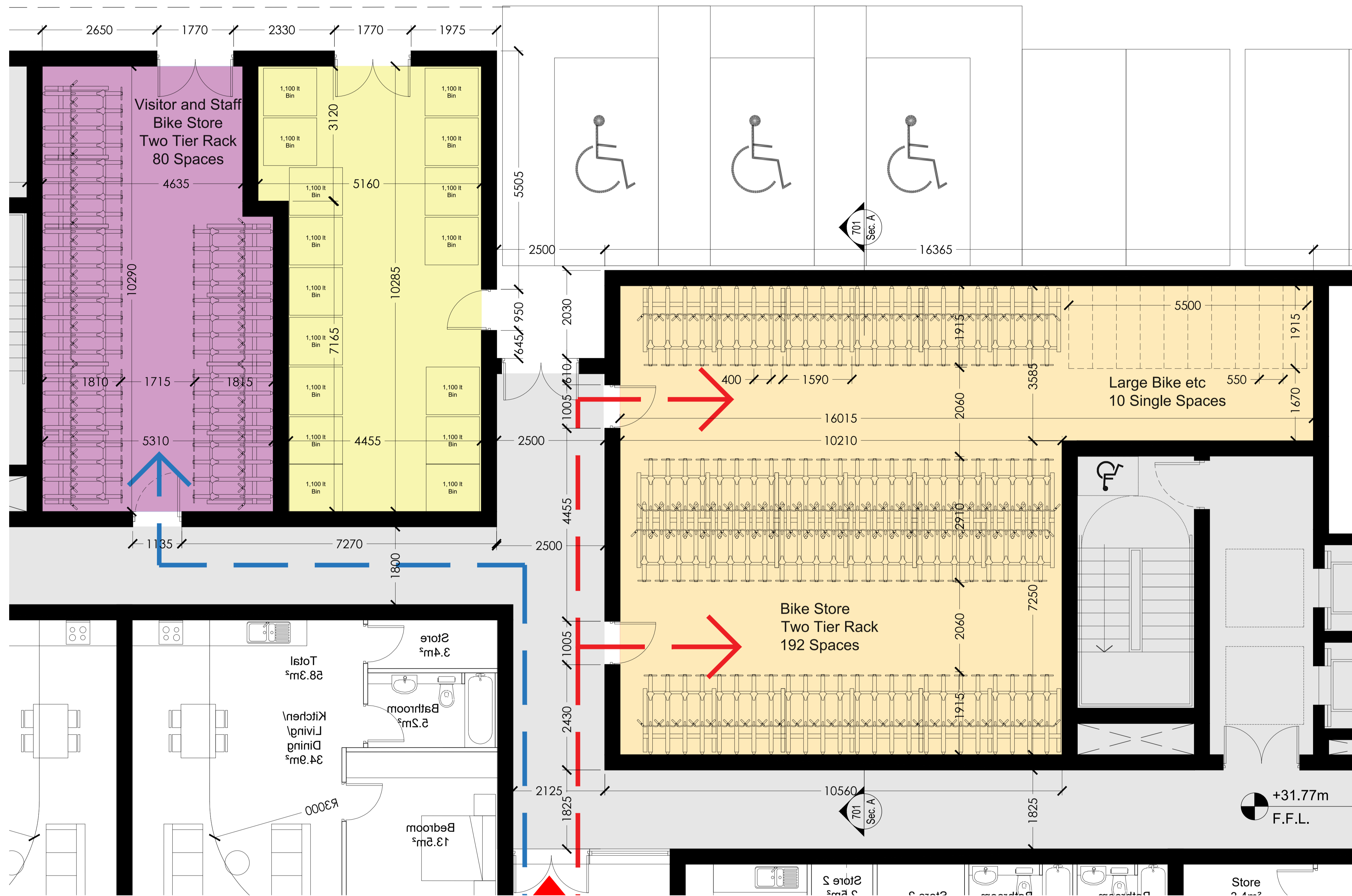
Residential, Visitor and Staff Bike Stores - Detail Plan
