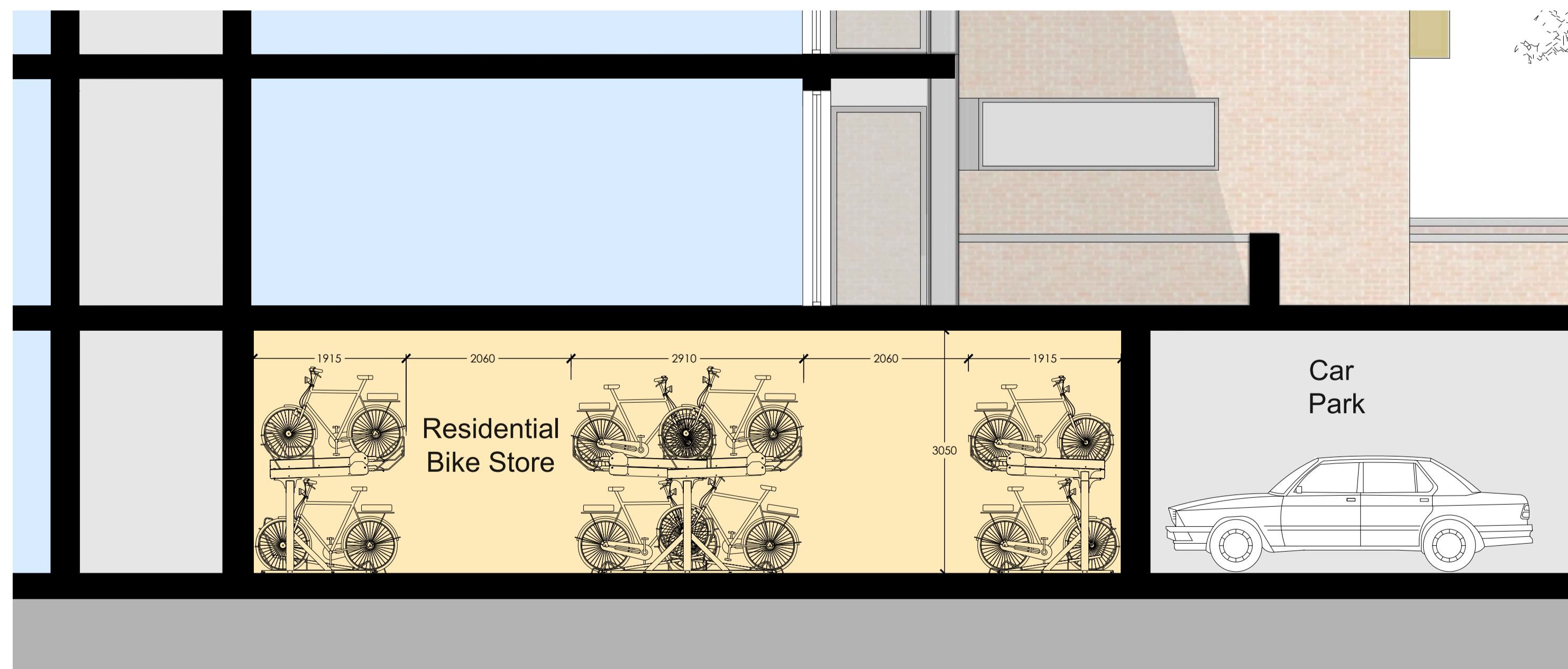
Residential Bike Store - Section A-A
