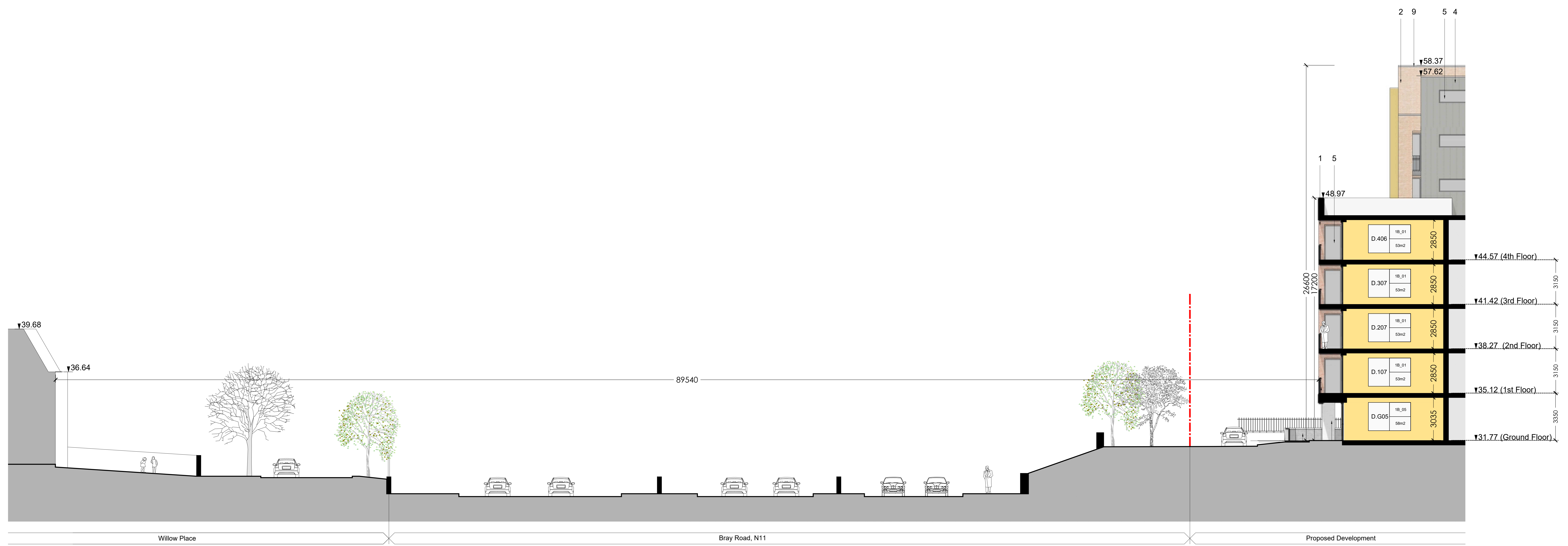
SECTION H-H (BUILDING D) Scale 1:100 @A0
