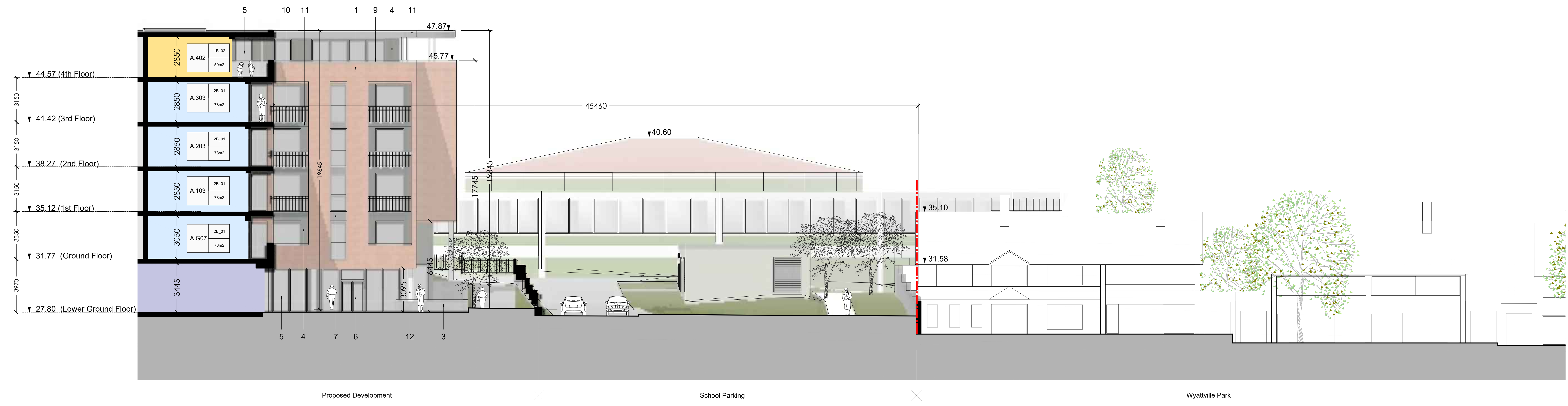
Section E-E (Building A) Scale 1:100@A0
