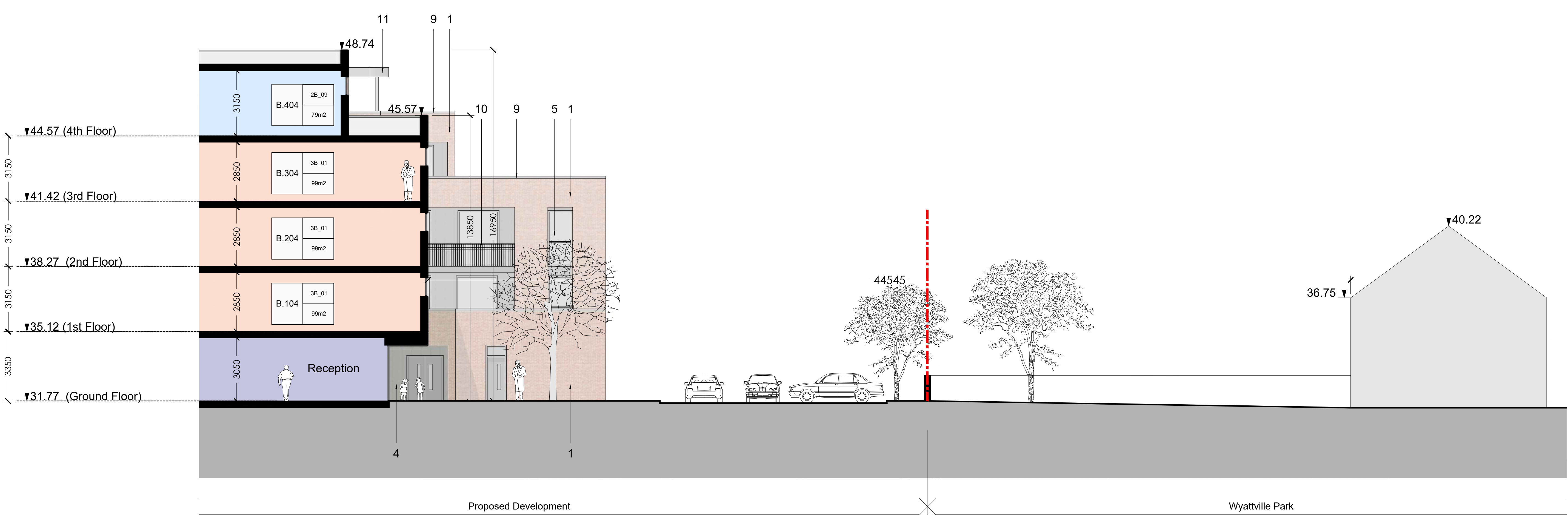
Section B-B (Building B) Scale 1:100@A0
